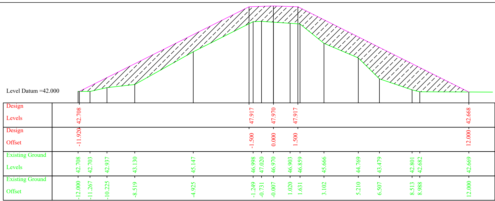
Chainage =750.000
