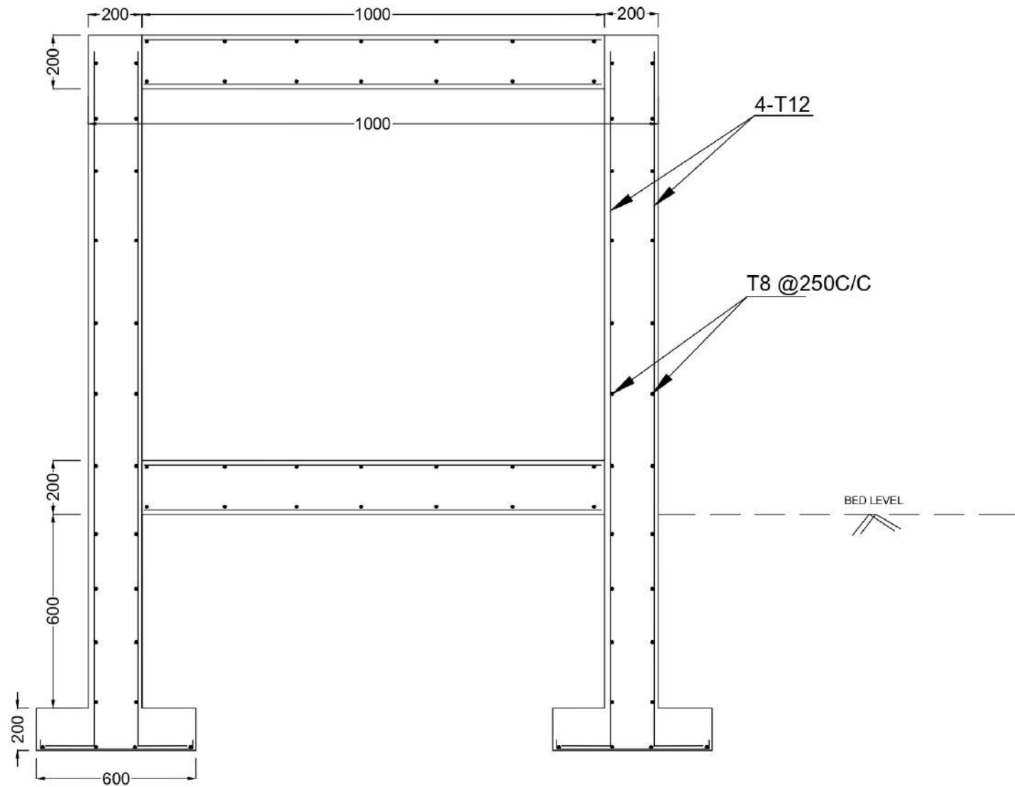
PLAN
