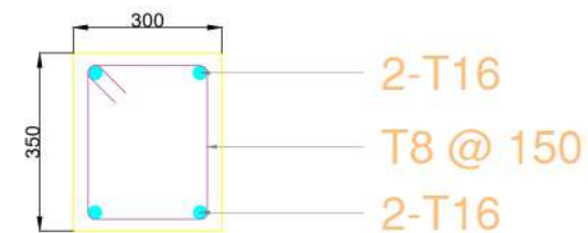
Plinth Beam Section
