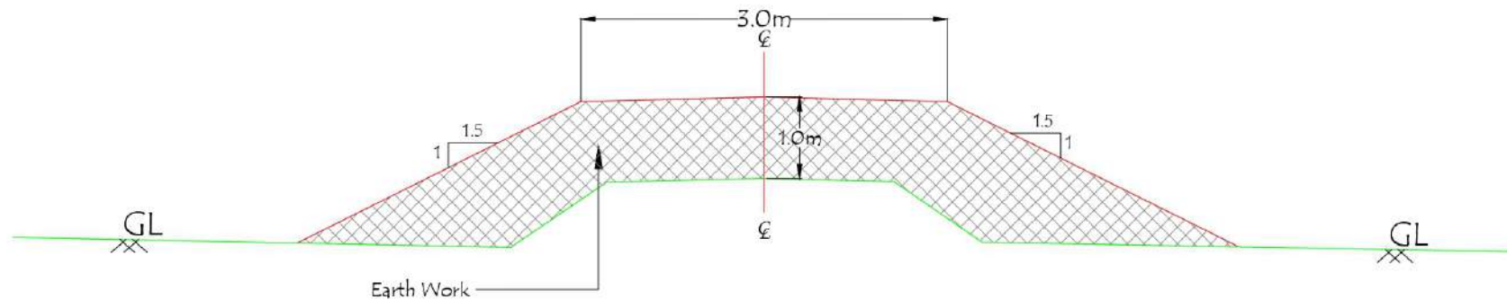
TYPICAL CROSS SECTION FOR BEEL EMBANKMENT LENGTH = 1600.00M
