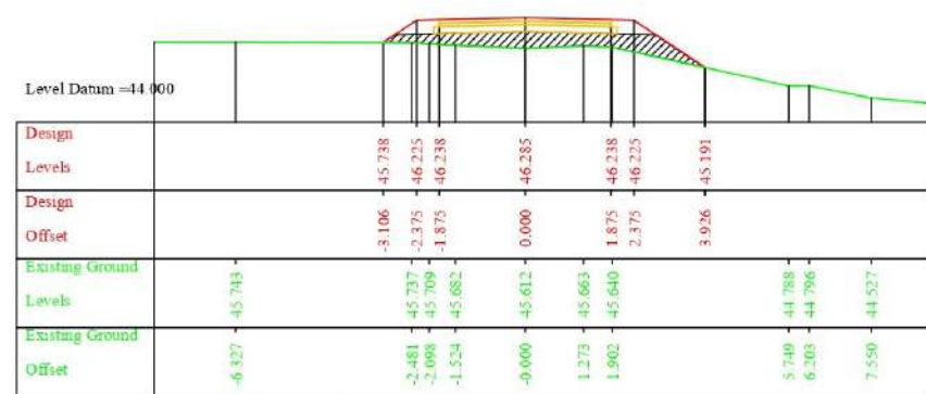
Chainage =210.000
