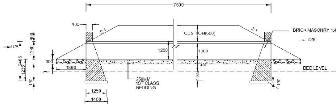
SECTION AT B-B
