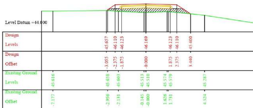
Chainage =240.000
