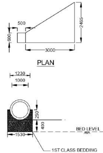
SECTION AT A-A (FOR PIPE BED)
