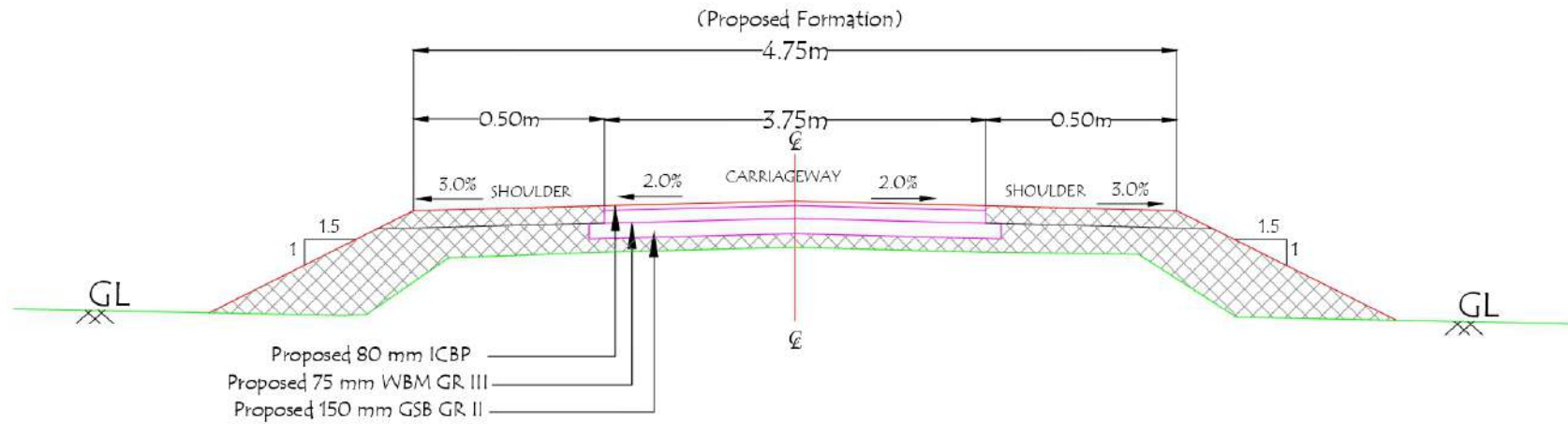
TYPICAL CROSS SECTION FOR APPROACH ROAD LENGTH= 610.00M
