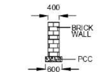
SECTION AT B-B
