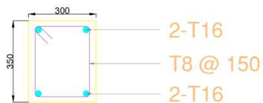
Beam above GL
